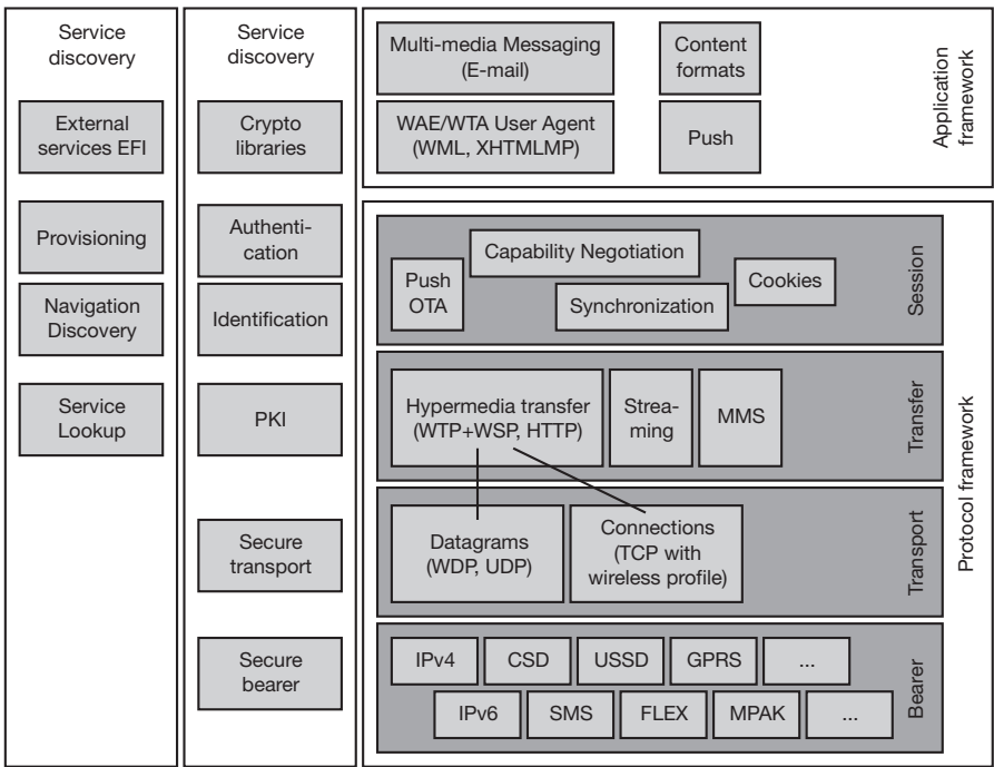
Figure 10.37 WAP 2.0 architecture
