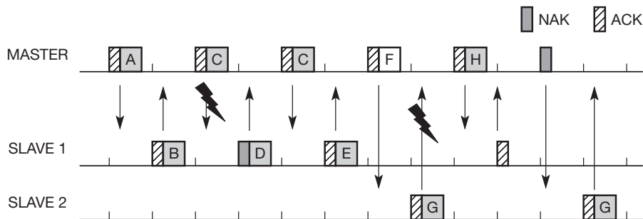
Figure 7.50 Error recovery
